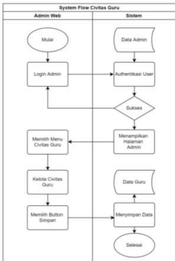
Gambar 6 System Flow Kelola Data Guru
