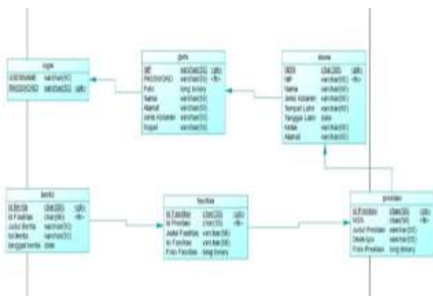
Gambar 2 Physical Data Model
