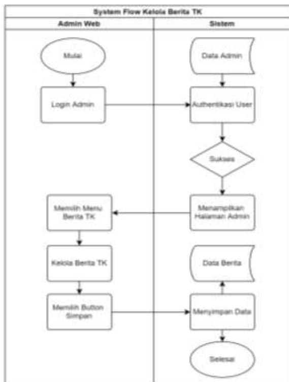
Gambar 5 System Flow Kelola Berita TK
