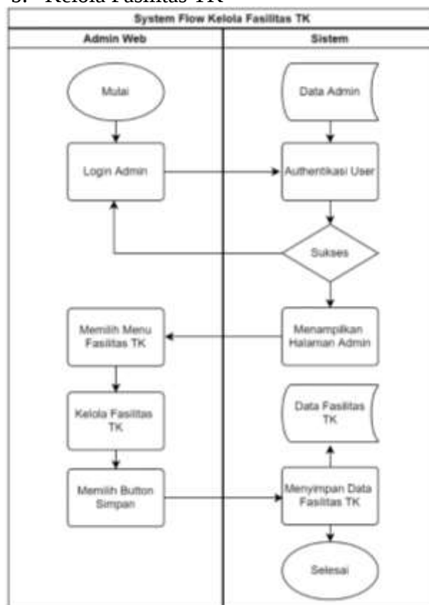
Gambar 4 System Flow Fasilitas TK
