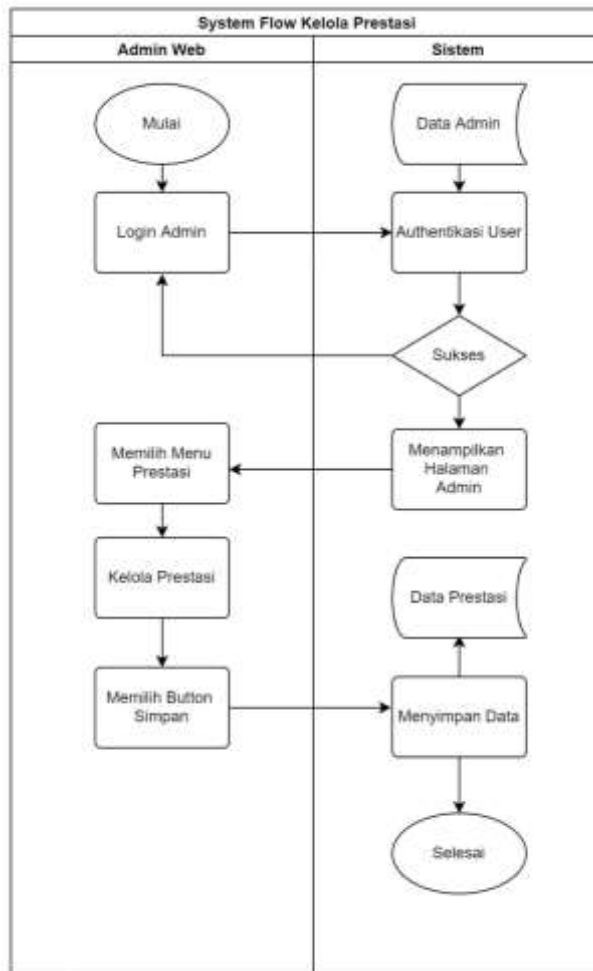
Gambar 7 System Flow Prestasi
