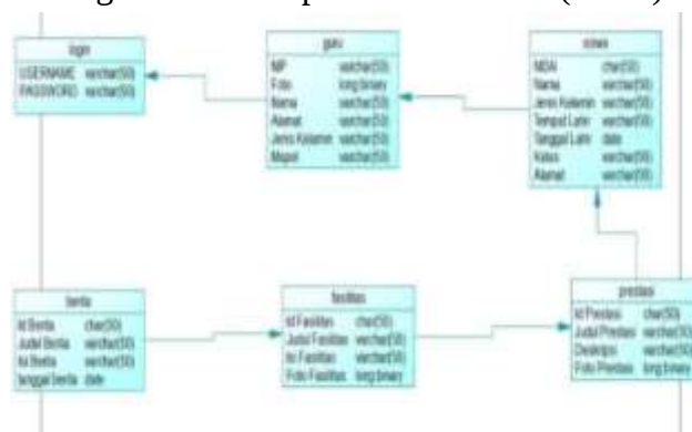
Gambar 1 Conceptual Data Model (CDM)
